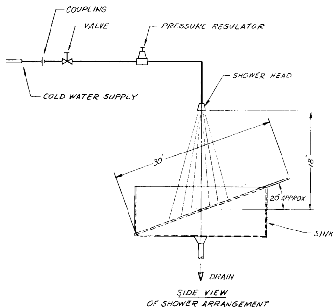
FIG. 1 Water Shower Exposure Test for Underlayment
