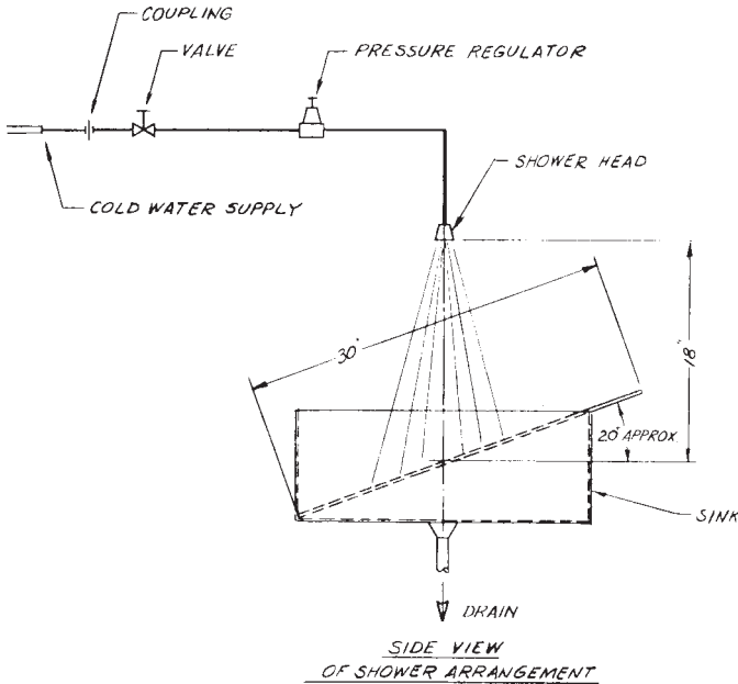
FIG. 1 Water Shower Exposure Test for Underlayment
