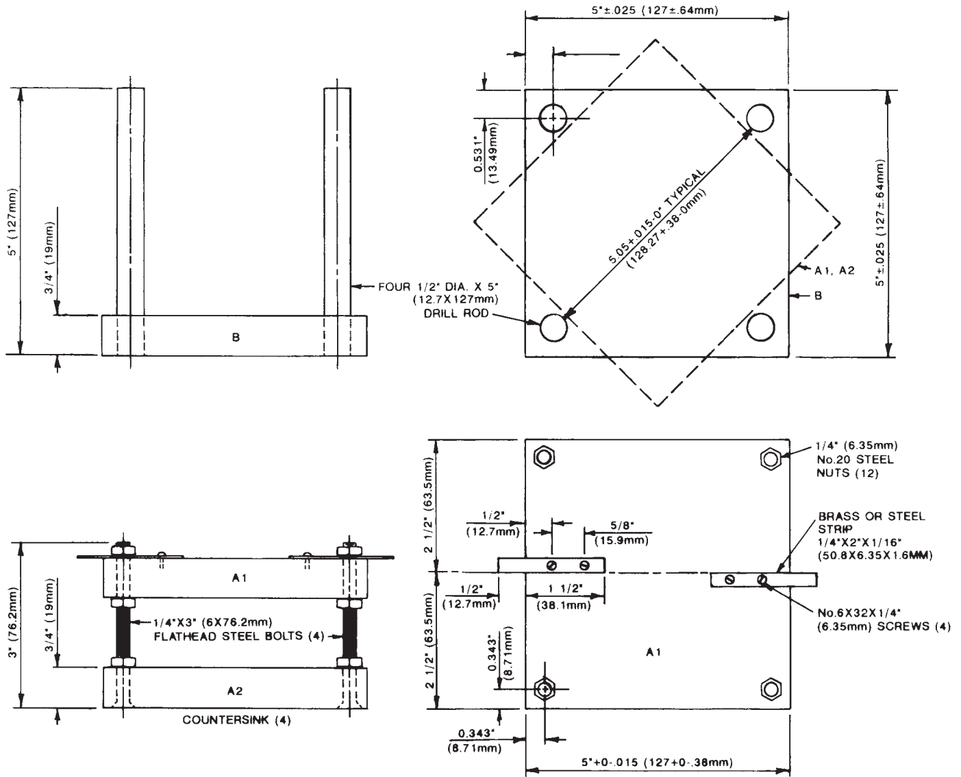
FIG. 2 Plastometer Details
