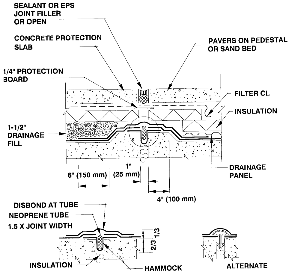
FIG. 15 Plaza Expansion Joint
