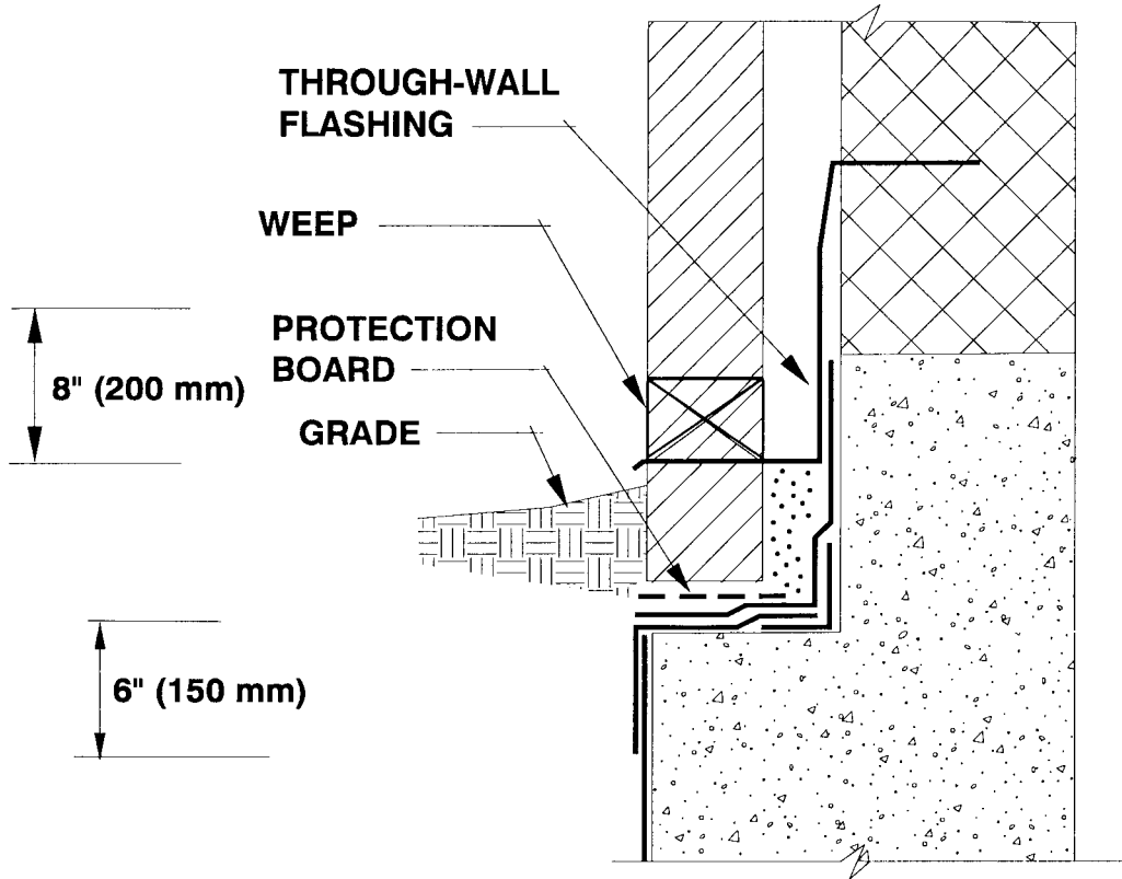
FIG. 10 Termination on Foundation with Brick Shelf
