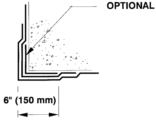
FIG. 6 Exterior Corner
