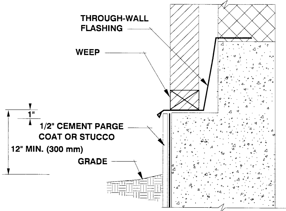
FIG. 11 Termination on Foundation Above Grade
