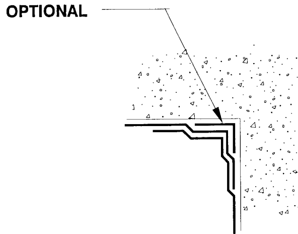
FIG. 7 Interior Corner
