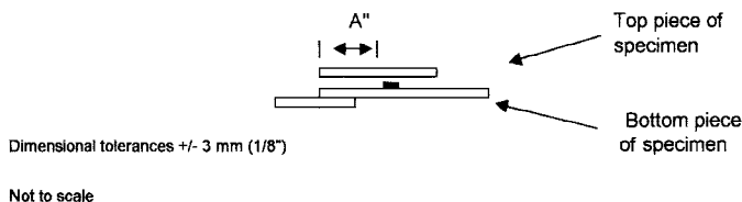
FIG. 3b Side View of Multi-ply Test Specimen
