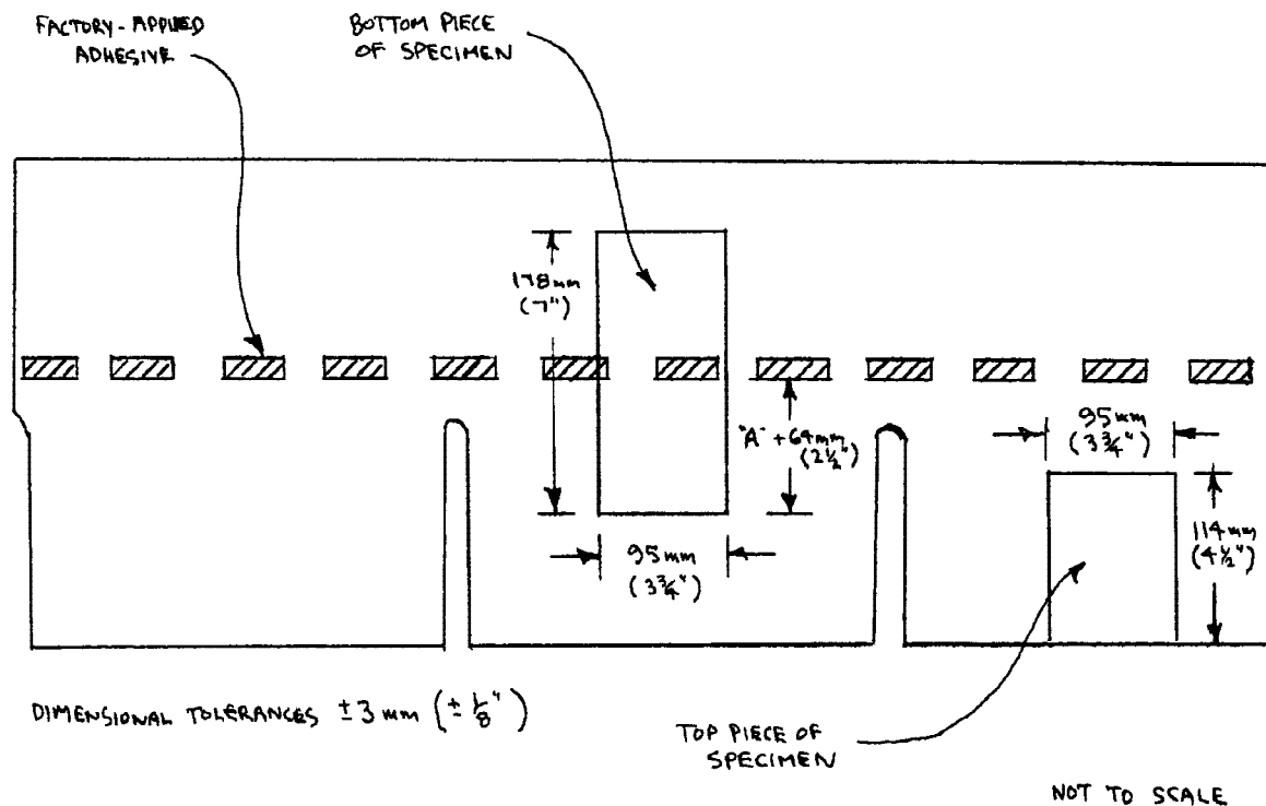
FIG. 2a Plan View of Shingle
