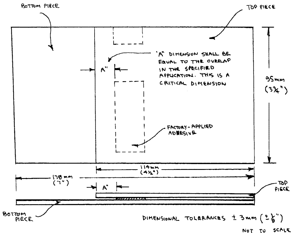
FIG. 3a Top and Side View of Test Specimen
