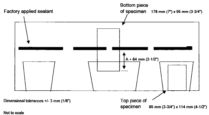
FIG. 2b Plan View of Multi-ply Shingle
