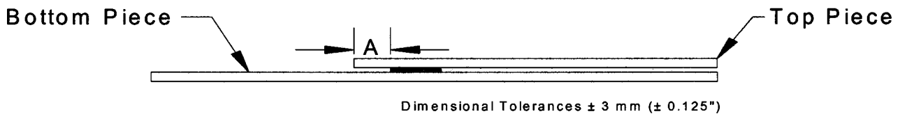
FIG. 4a Top and Side View of Test Specimen—Procedure A
