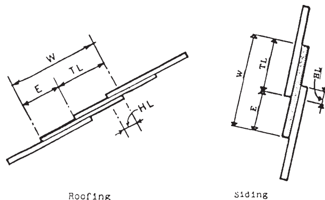
Terminology E—Exposure TL—Toplap HL—Head lap W—Width for strip shingles or length for individual shingles
