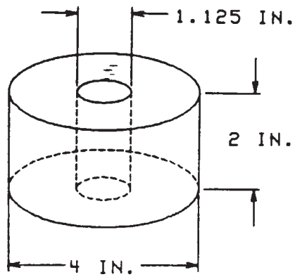
FIG. 1 Test Specimen
