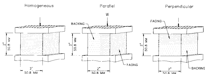
FIG. 1 Loading Position
