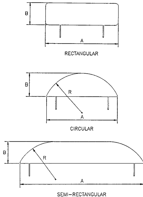
FIG. 1 Flatjack Configurations
