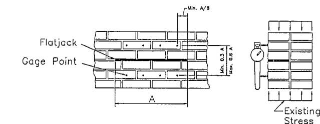
FIG. 2 Flatjack Test Setup for In Situ Stress Measurement
