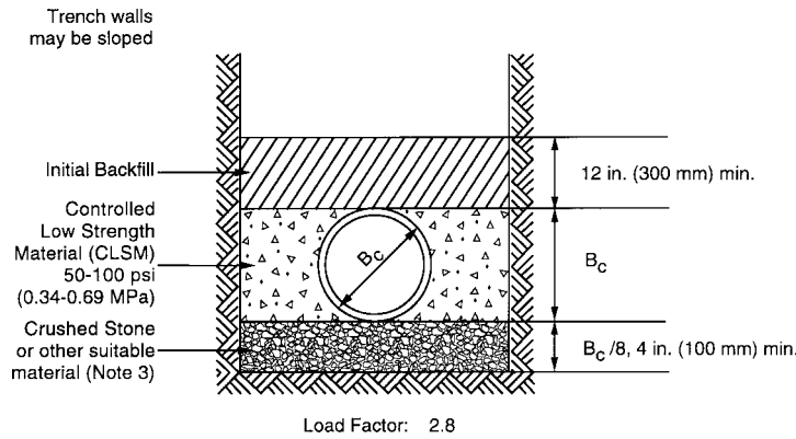
FIG. 6 Controlled Low Strength Material (CLSM)
