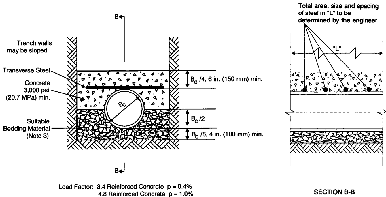
FIG. 7 Concrete Cradle
