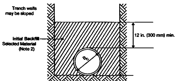
Load Factor: 1.1 Flat or Restored Trench Bottom
