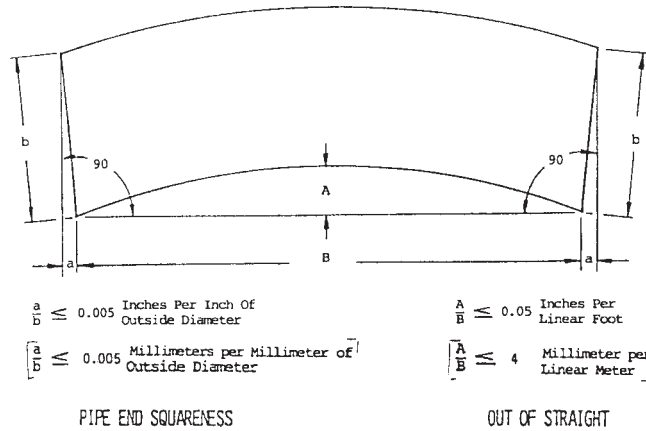
NOTE 1—Illustration is exaggerated to show dimensions. FIG. 1 Pipe End Squareness and Out of Straight
