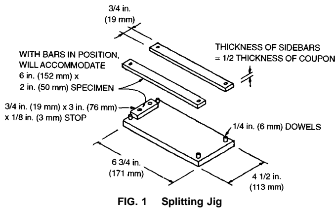
FIG. 1 Splitting Jig
