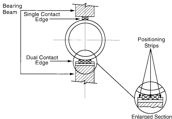
FIG. 2 Loading Apparatus
