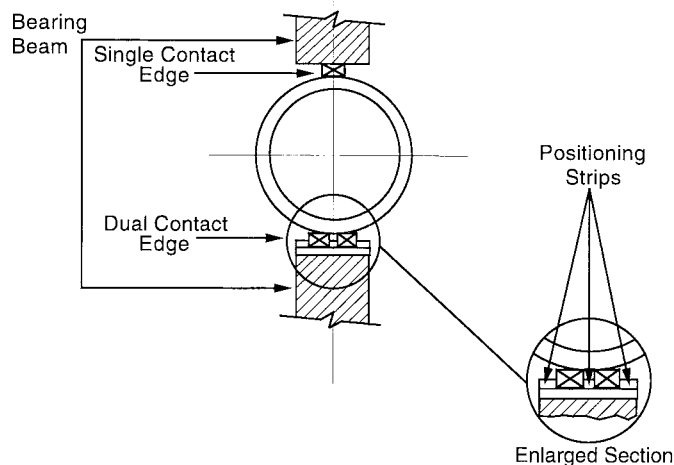
FIG. 2 Loading Apparatus
