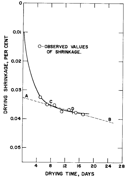
NOTE—The interval CD is 6 days on the time scale and % on the shrinkage scale. Point D defines equilibrium shrinkage value.
