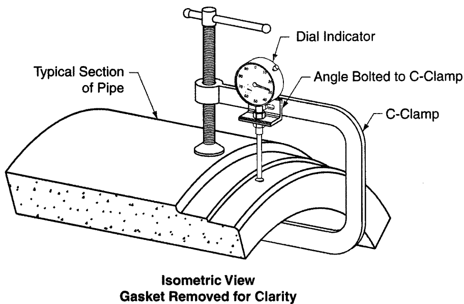
FIG. 11 Dial Indicator
