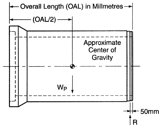
FIG. 10 Simplified Center of Gravity of Pipe
