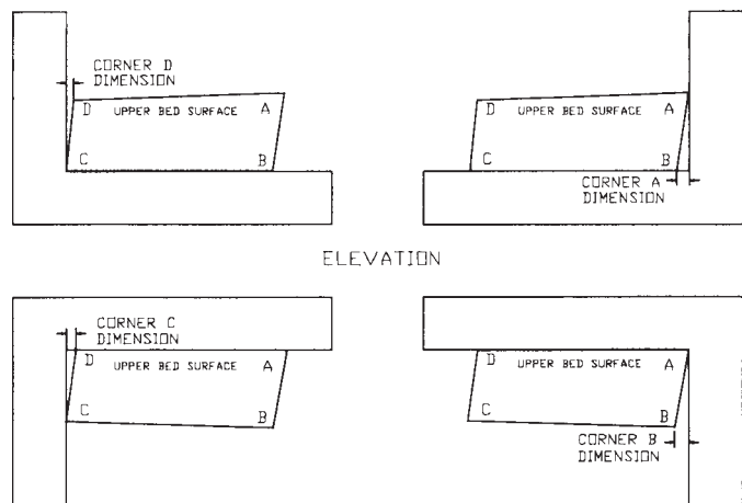
FIG. 4 Out-of-Square Measurements
