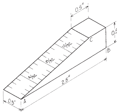
FIG. 1 Measuring Wedge
