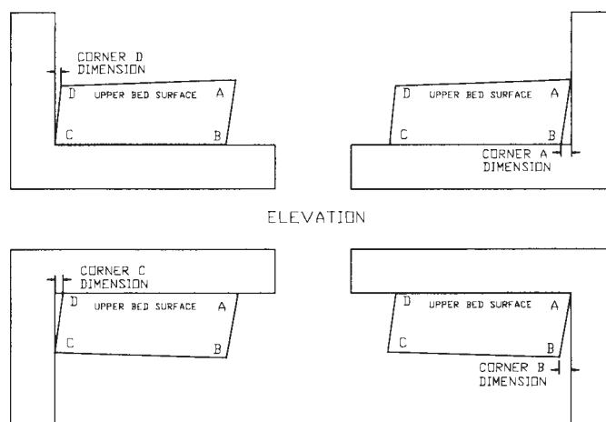
FIG. 4 Out-of-Square Measurements
