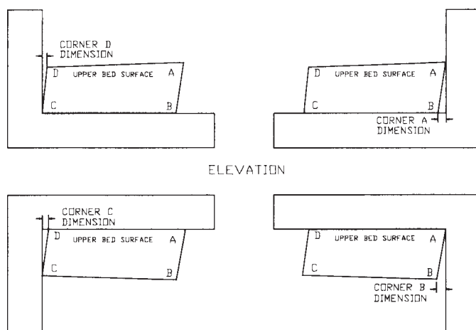
FIG. 4 Out-of-Square Measurements
