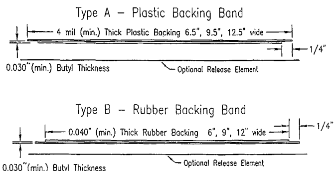
FIG. 3 Sealing Band Type III (Not to Scale)
