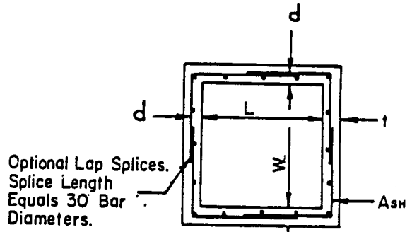
FIG. X1.2 Section AA
