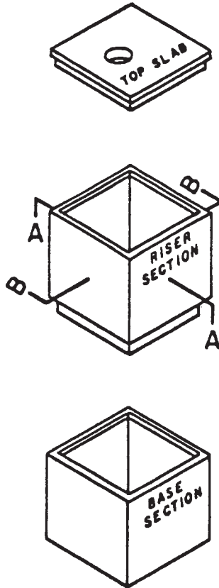
FIG. X1.1 Typical Assembly
