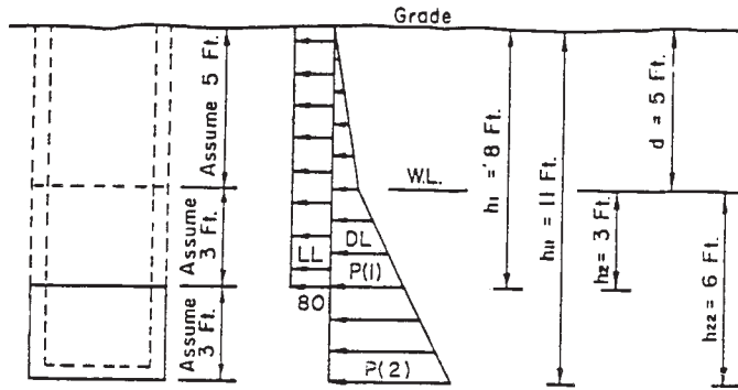
FIG. X2.2 Load Diagram
