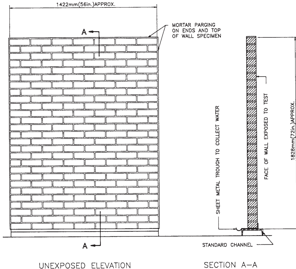
UNEXPOSED ELEVATION SECTION A-A FIG. 3 Typical Brick Masonry Test Specimen
