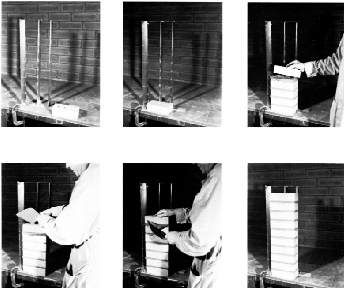
FIG. 3 Use of a Jig to Align One Face of a Prism to a Plane
