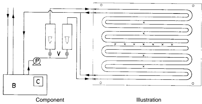
FIG. A2.1 Assembled Metal-Screen Heater Apparatus Without Perimeter Insulation
