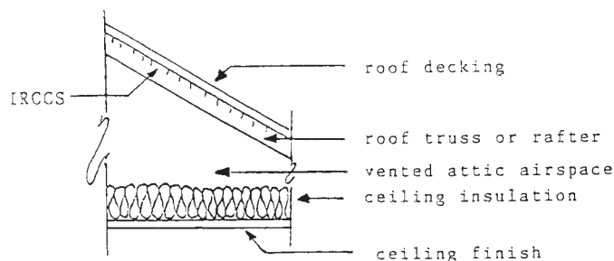
NOTE 1—Apply IRCCS to cover the exposed roof deck area. The low-emittance surface of the IRCCS must face the interior of the attic.
