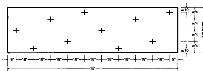
FIG. 3 Thickness Measurement Locations – Full Roll
