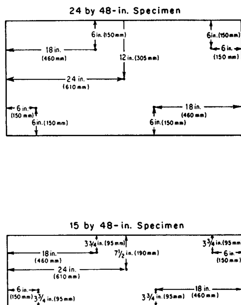
FIG. 2 Thickness Measurement Locations
