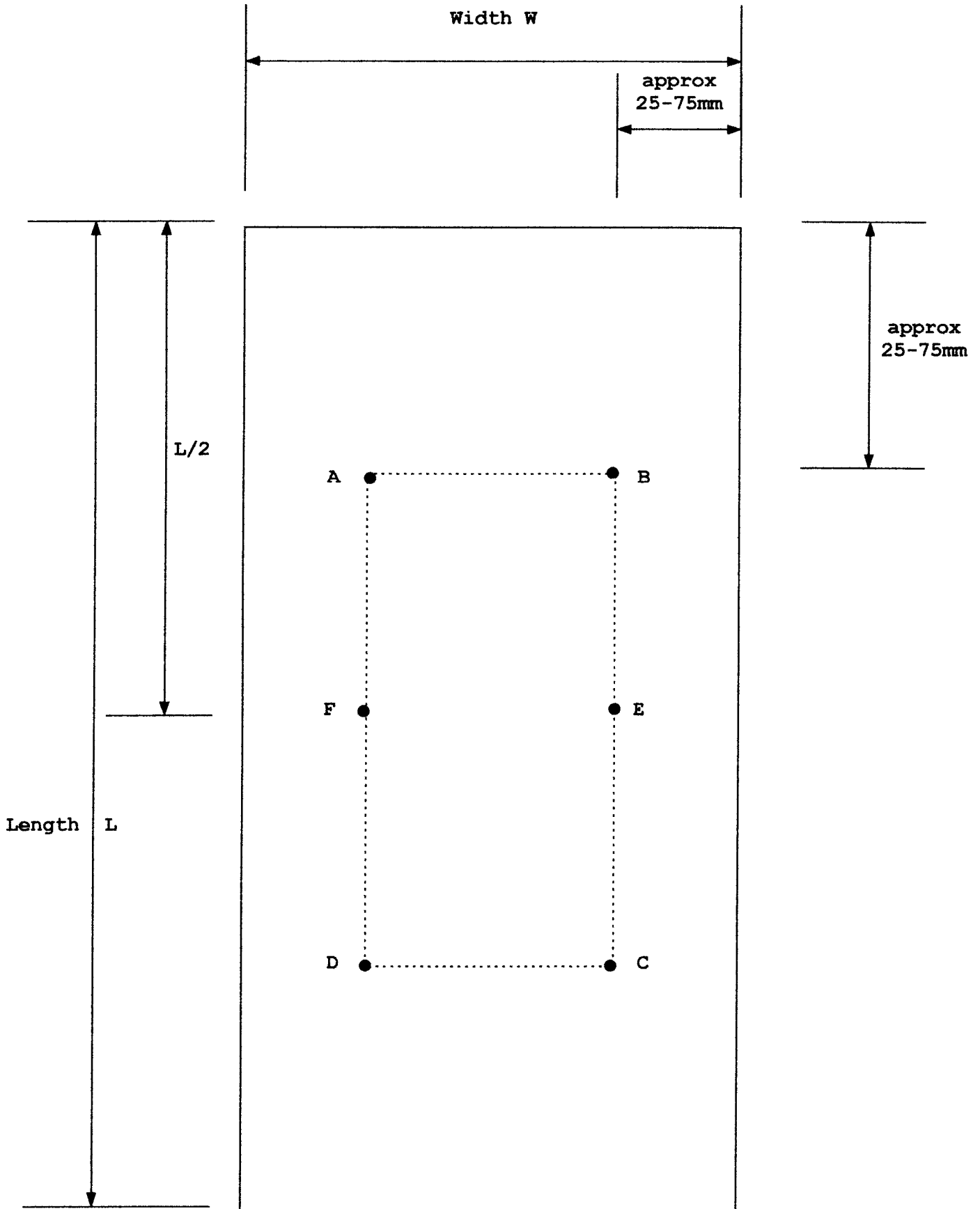
FIG. 1 Specimen Measurement
