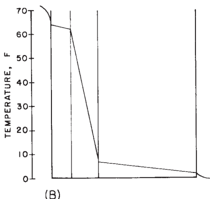
FIG. A1.1 Vapor Pressure and Temperature Gradients of Building Wall (6)
