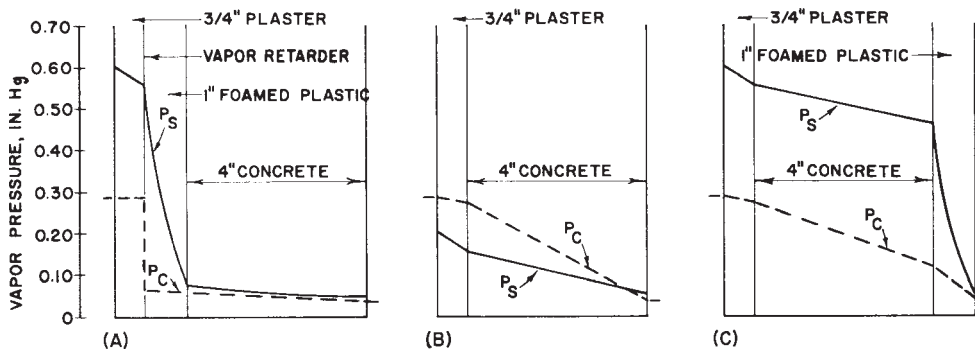
FIG. X1.2 Vapor Pressure Gradients of Modified Building Wall (6)
