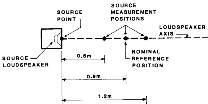
FIG. 3 Measurement Positions for Reference Levels
