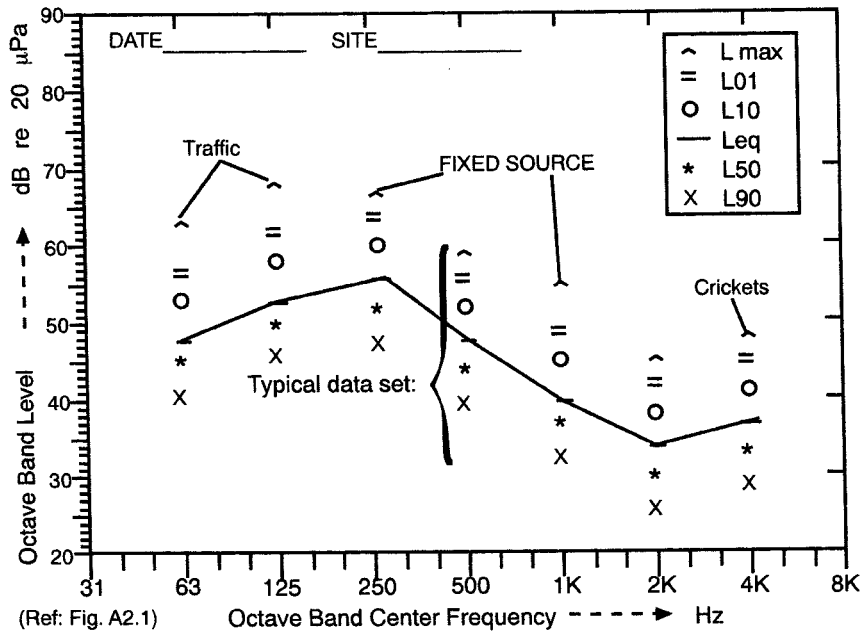
FIG. A3.2 Typical Octave Band Spectrum Graph
