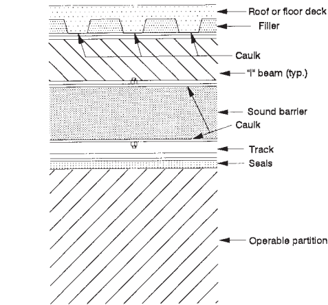
FIG. 1 Recommended Ceiling Barrier Installation
