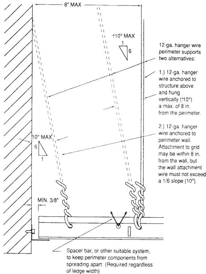
FIG. 3 Light to Moderate Treatment of Cross Runners and Main Runners at Terminal Ends When Support Ledge of Perimeter Closure is Less Than Minimum \frac{3}{8} in.
