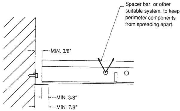
FIG. 1 Light to Moderate Treatment of Cross Runners, Main Runners, and Wall Closures at Terminal Ends
