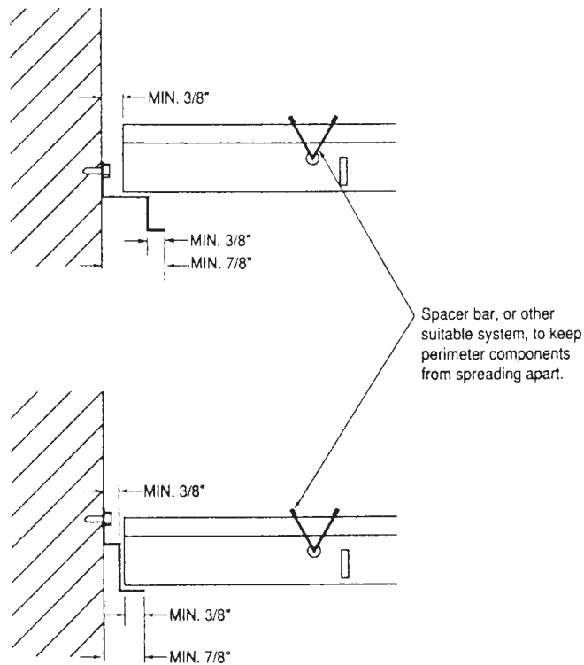
FIG. 2 Light to Moderate Treatment of Cross Runners and Main Runners at Terminal Ends When Using Reveal (Shadow) Edge Wall Closures
