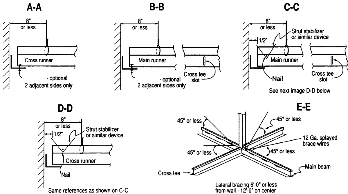
FIG. 4 Moderate to Severe Treatment
