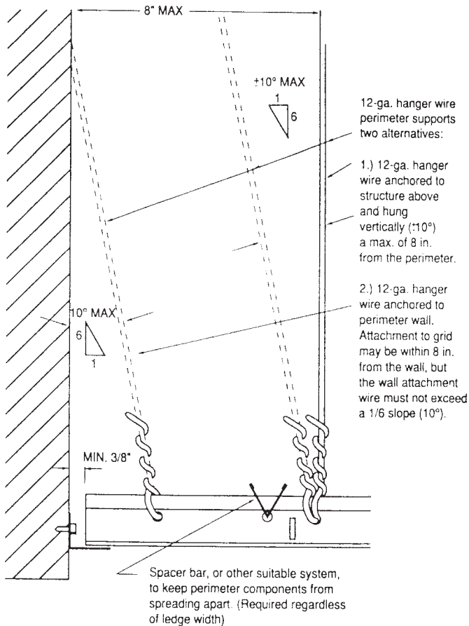
FIG. 3 Light to Moderate Treatment of Cross Runners and Main Runners at Terminal Ends When Support Ledge of Perimeter Closure is Less Than Minimum 3/8 in.
