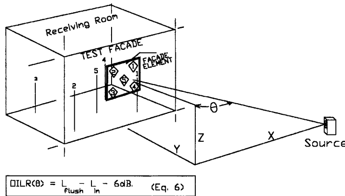
FIG. 3 Geometry—Flush Method
