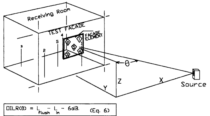
FIG. 3 Geometry—Flush Method
