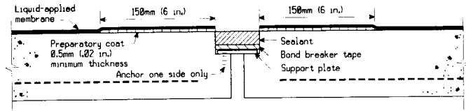
FIG. 8 Typical Expansion Joint (see 10.4.4.3 and 14.5.6)
