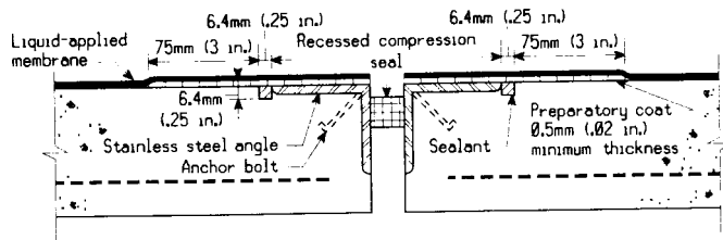
FIG. 8 Typical Expansion Joint (see 10.4.4.3 and 14.5.6)
