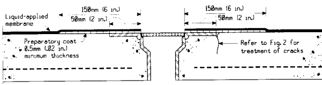
FIG. 11 Termination at Drain with a Wide Flange (see 10.4.2 and 14.6.2)
