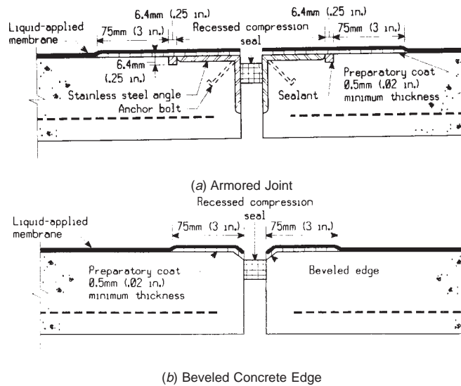
FIG. 9 Typical Compression Seal Joint (see 10.4.4.3 and 14.5.7)
