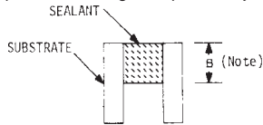
(b) Sideview of Test Specimen with Spacer Removed SEALANT SHAPE 12.7 by 12.7 by 50.8 mm (0.5 by 0.5 by 2.0 in.)
