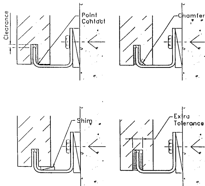
FIG. 5 Point Loading Prevention (continued) (continued)
