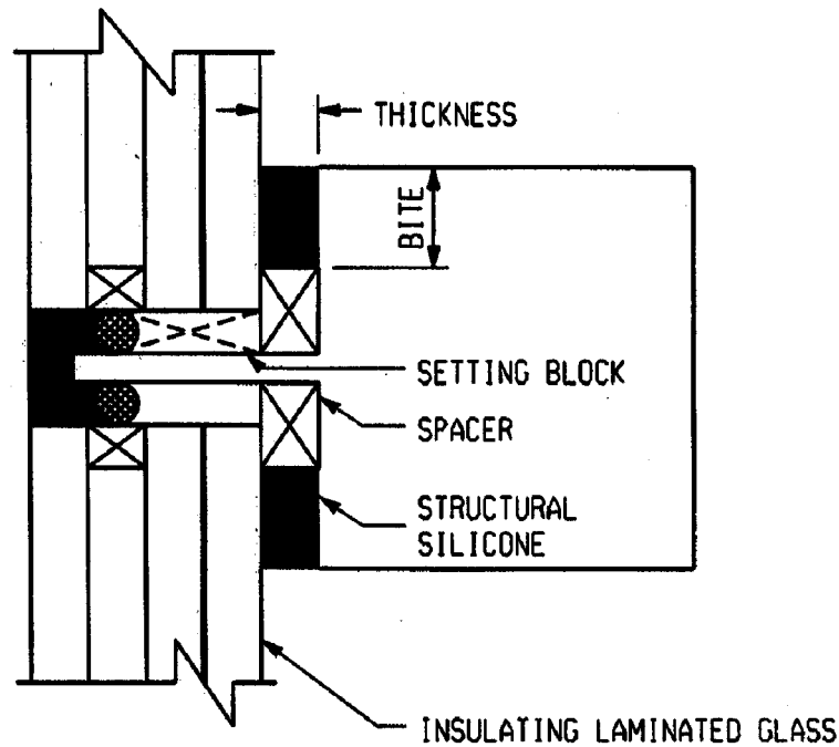
FIG. 3 Typ General Missile Impact Detail with Insulating Laminated Glass
