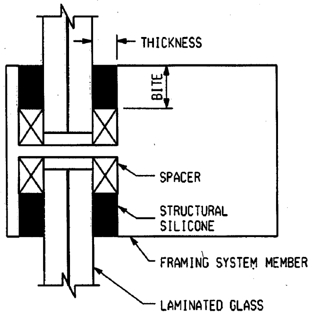
FIG. 5 Typ Genericat Missile Impact or Bomb Blast Detail with Laminated Glass
