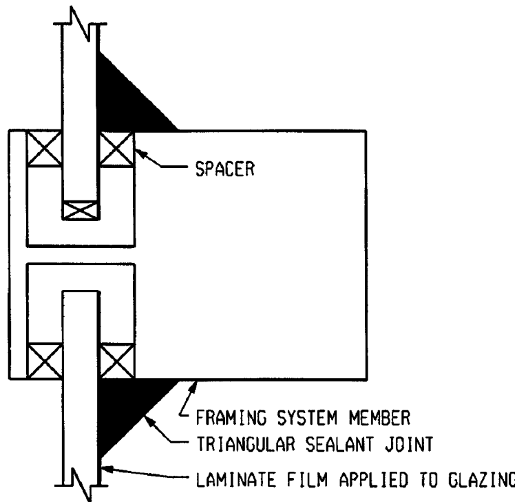
FIG. 7 Typ General Retrofit Impact Resistant Detail with Monolithic Glass and Laminate
