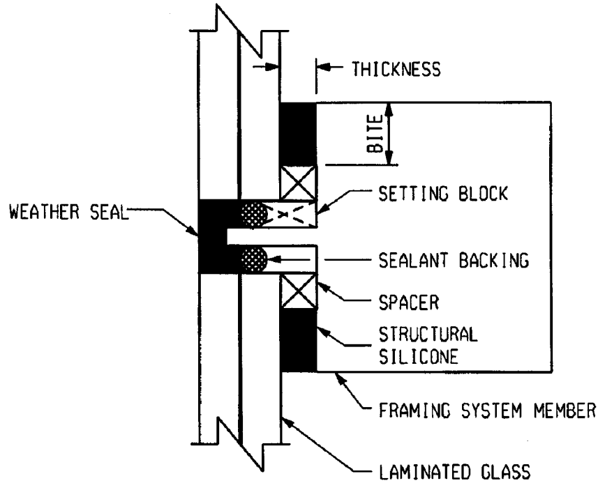
FIG. 2 Typ General Missile Impact Detail with Laminated Glass
