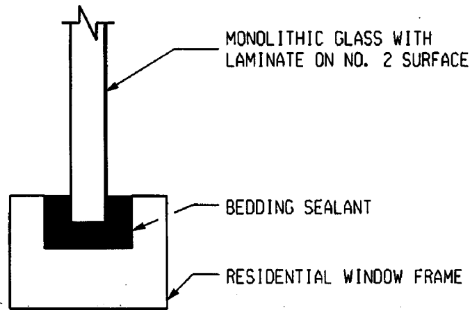
FIG. 8 Typ General Residential Impact Resistance Detail
