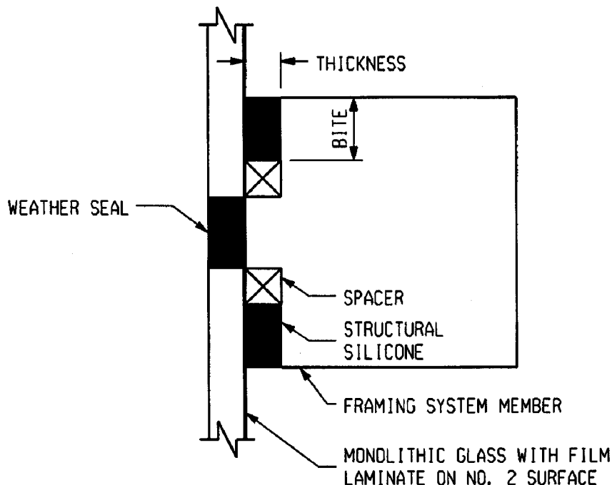
FIG. 1—Typ Generic Missile Impact Detail with Monolithic Glass with Laminate
