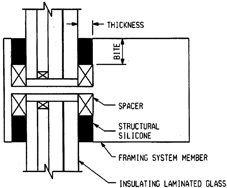
FIG. 6 Typ General Missile Impact or Bomb Blast Detail with Insulating Laminated Glass
