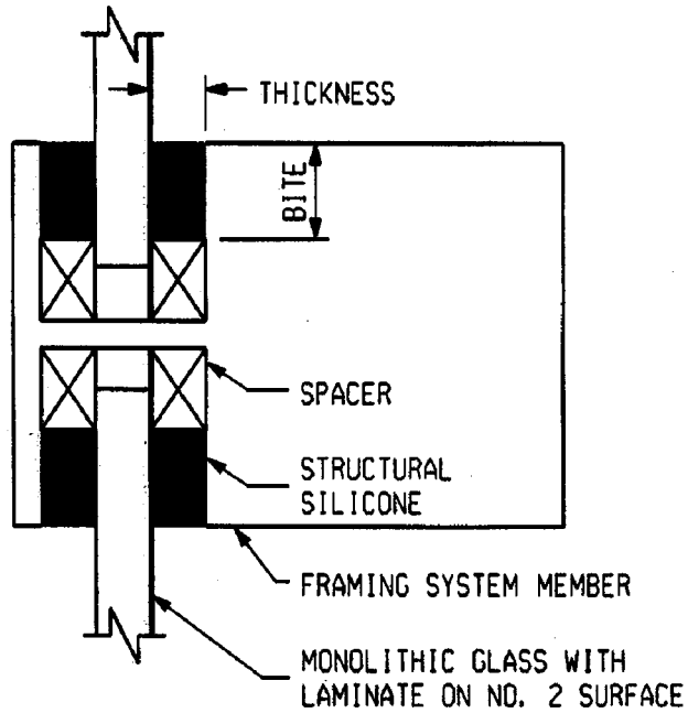
FIG. 4 Typ Genericat Missile Impact or Bomb Blast Detail with Monolithic Glass with Laminate
