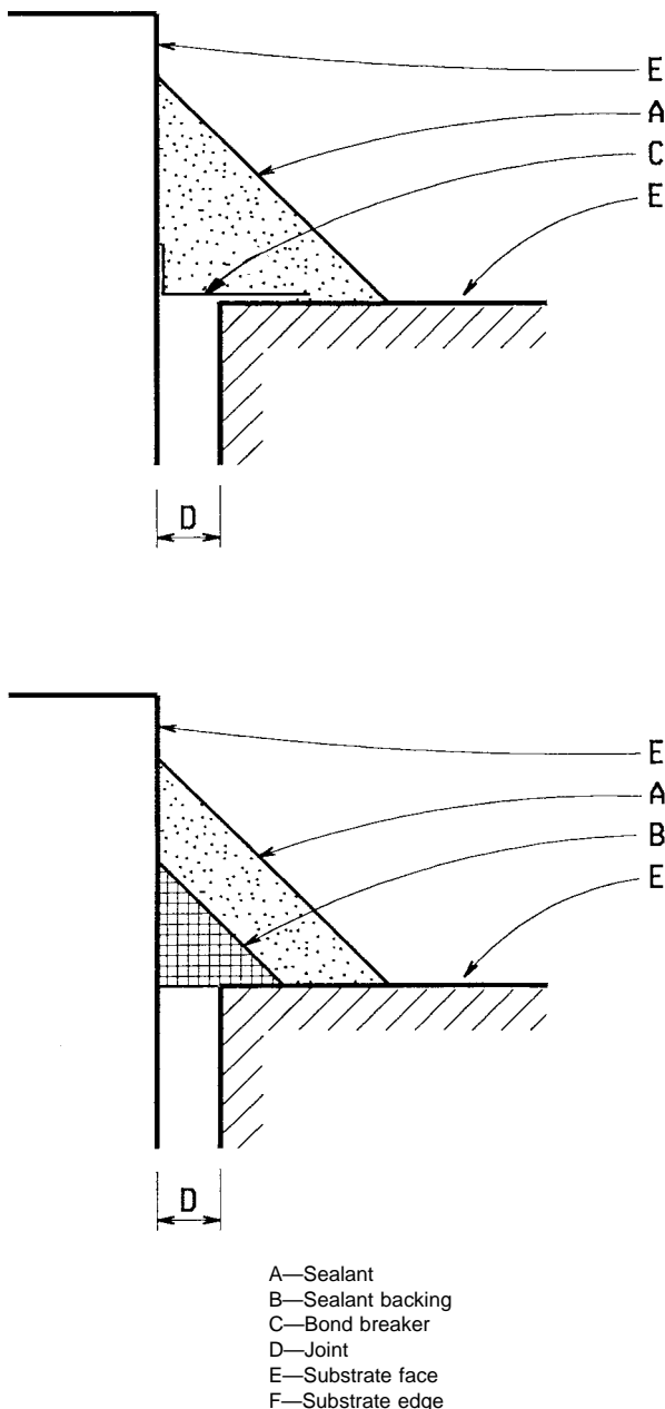
FIG. 3 Fillet Sealant Joints
