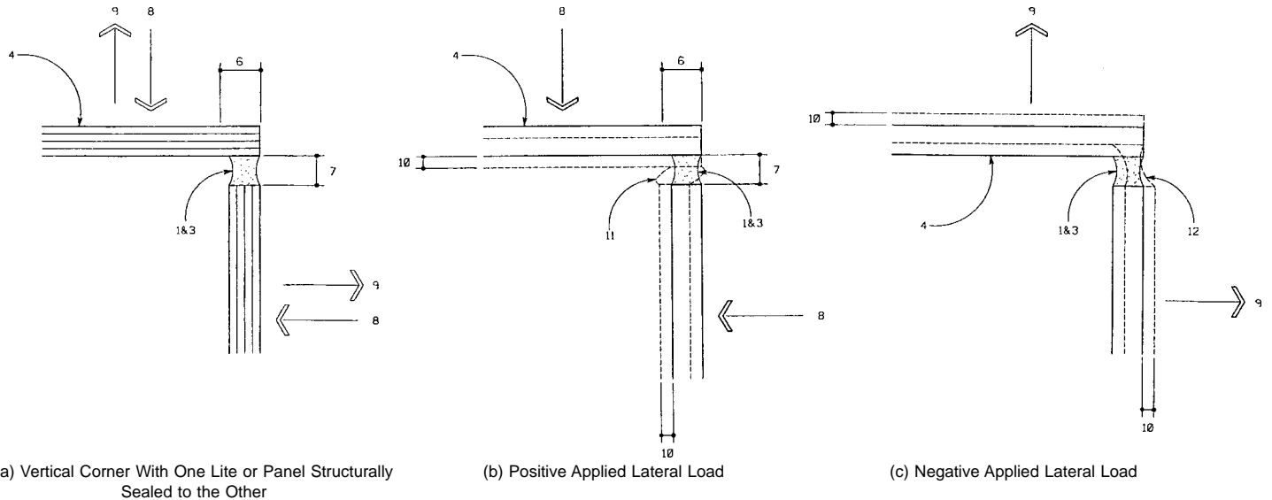
FIG. 6 Applied Load Transfer at a Vertical Corner Structural Sealant Joint (see Fig. 5 for Legend)
