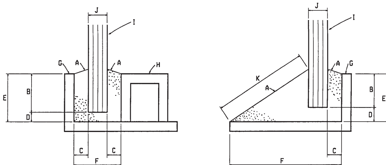
Channel Glazing
