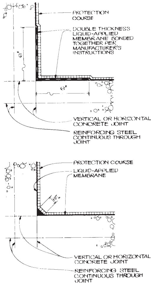
FIG. 14 Turnup Details at Reinforced Joint (see 18.6)
