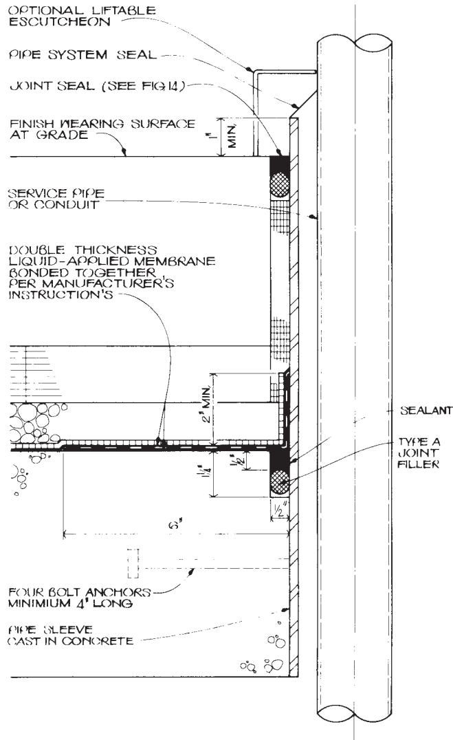
FIG. 6 Termination at Pipe Penetrations (see 7.8.3.3 and 178.9)
