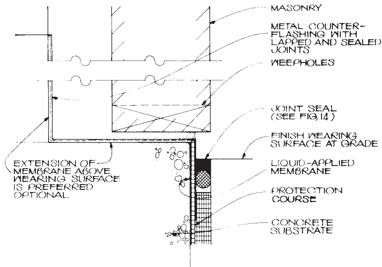
FIG. 4 Terminal Condition with Masonry Above Finish Wearing Surface at Grade (see-7 8.3.1)
