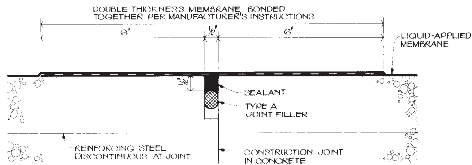
FIG. 8 Treatment of Nonreinforced Butted-Joint in Concrete Slab (see 7.8.4.2)
