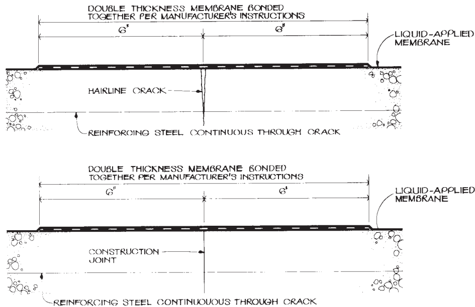
FIG. 7 Treatment of Reinforced Cracks and Joints in Concrete Slab (see 7.8.4.1)
