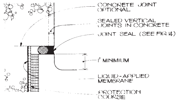
FIG. 2 Terminal Condition Above Finish Grade on Concrete Wall (see-7 8.3.1)
