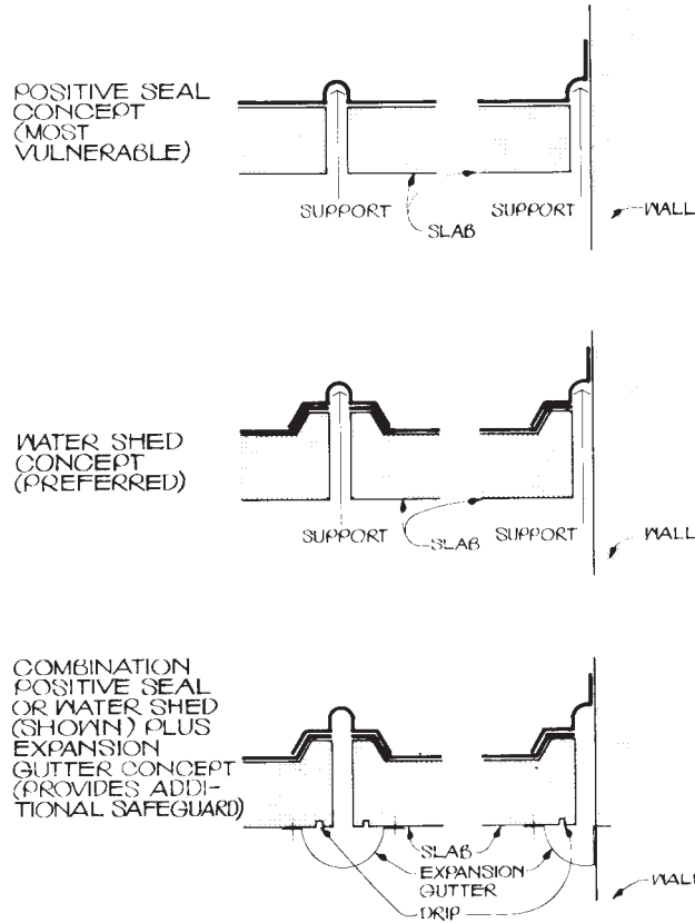
FIG. 9 Schematic Expansion Joint Concepts at Membrane Level
