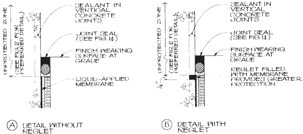
FIG. 3 Terminal Conditions on Concrete Wall Below Finish Wearing Surface at Grade (see-7 8.3.1)
