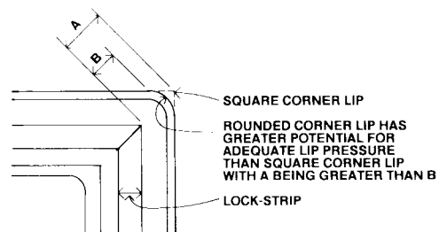
FIG. 9 Gasket Corner Design Features
