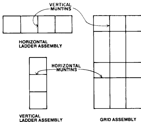
FIG. 3 Gasket Systems
